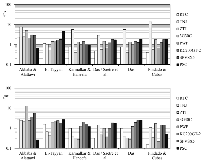
Figure 13. Comparison of the different explicit models studied, computationally fitted (best fit) to the I-V curves selected for the benchmark (Table 2). Normalized RMSE, \zeta , (Equation (37)), and normalized RMSE within \pm 5\% of V_{oc} around the maximum power point, \zeta^* . See also Tables 3–8.
