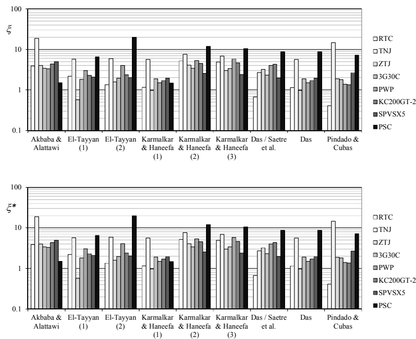
Figure 12. Comparison of the different explicit models studied, analytically fitted to the I-V curves selected for the benchmark (Table 2). Normalized RMSE, \zeta , (Equation (37)), and normalized RMSE within \pm 5\% of V_{oc} around the maximum power point, \zeta^* . See also Tables 3–8. El-Tayyan (1) indicates Equation (13), whereas El-Tayyan (2) refers to Equation (18). Karmalkar & Haneefa (1) indicates Equation (20), Karmalkar & Haneefa (2) refers to Equation (22), and Karmalkar & Haneefa (3) indicates Equation (24).
